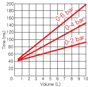
DVX40 Pressurization
