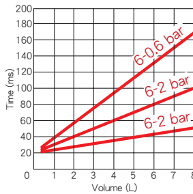
DVX40 Depressurization (P,A port G1 1/4)
