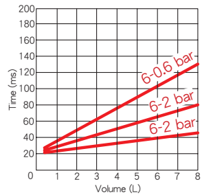
DVX40 Depressurization (P,A port G1 1/2)
