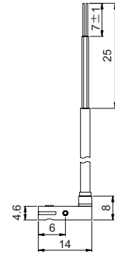
DTH-F9BV / DTH-F9NV / DTH-F9PV 外型尺寸
